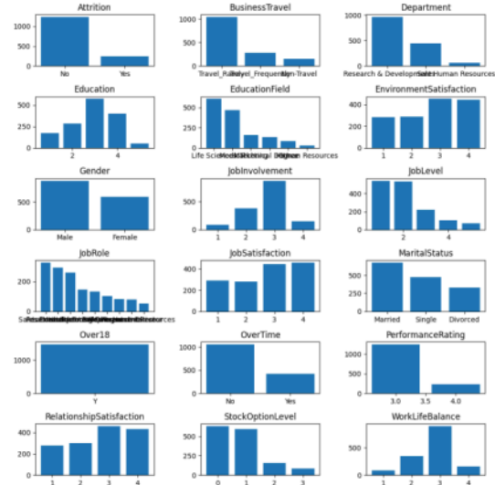
Fig. 3. EDA Visualization in Categorical Column
