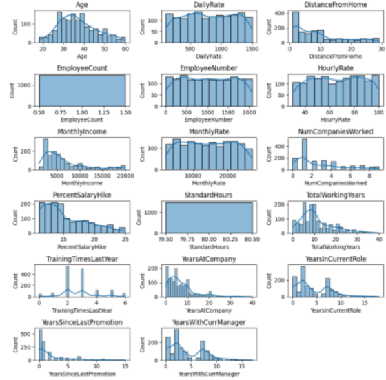
Fig. 2. EDA Visualization in Numerical Column
